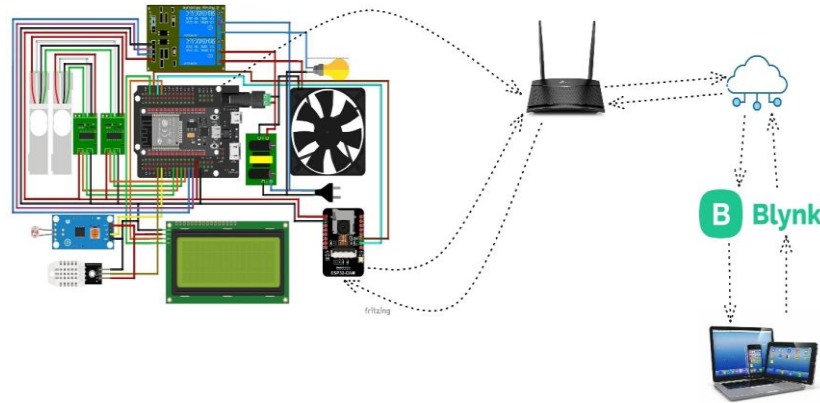
Figure 2 Circuit Diagram
